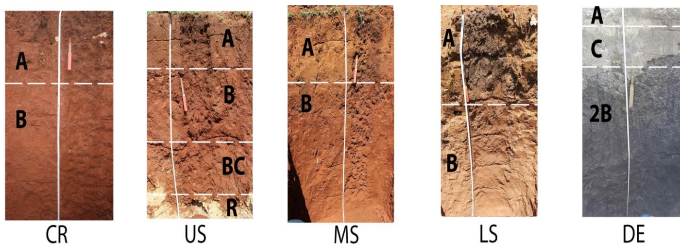
Figure 2. Profiles of the representative pedons.
